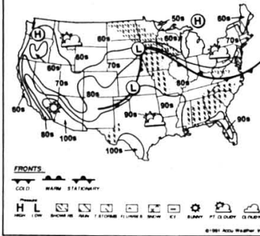
Expected sky conditions for tomorrow
